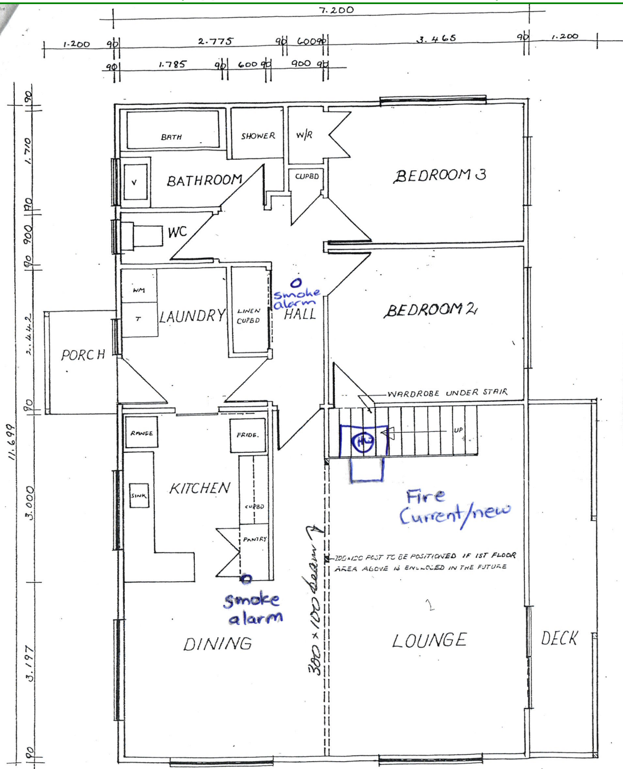
GROUND FLOOR PLAN 84.23 sqm (906.3 sq')
