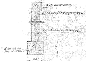
SECTION C.I. 1/4\"/>
