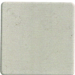
Ariel
