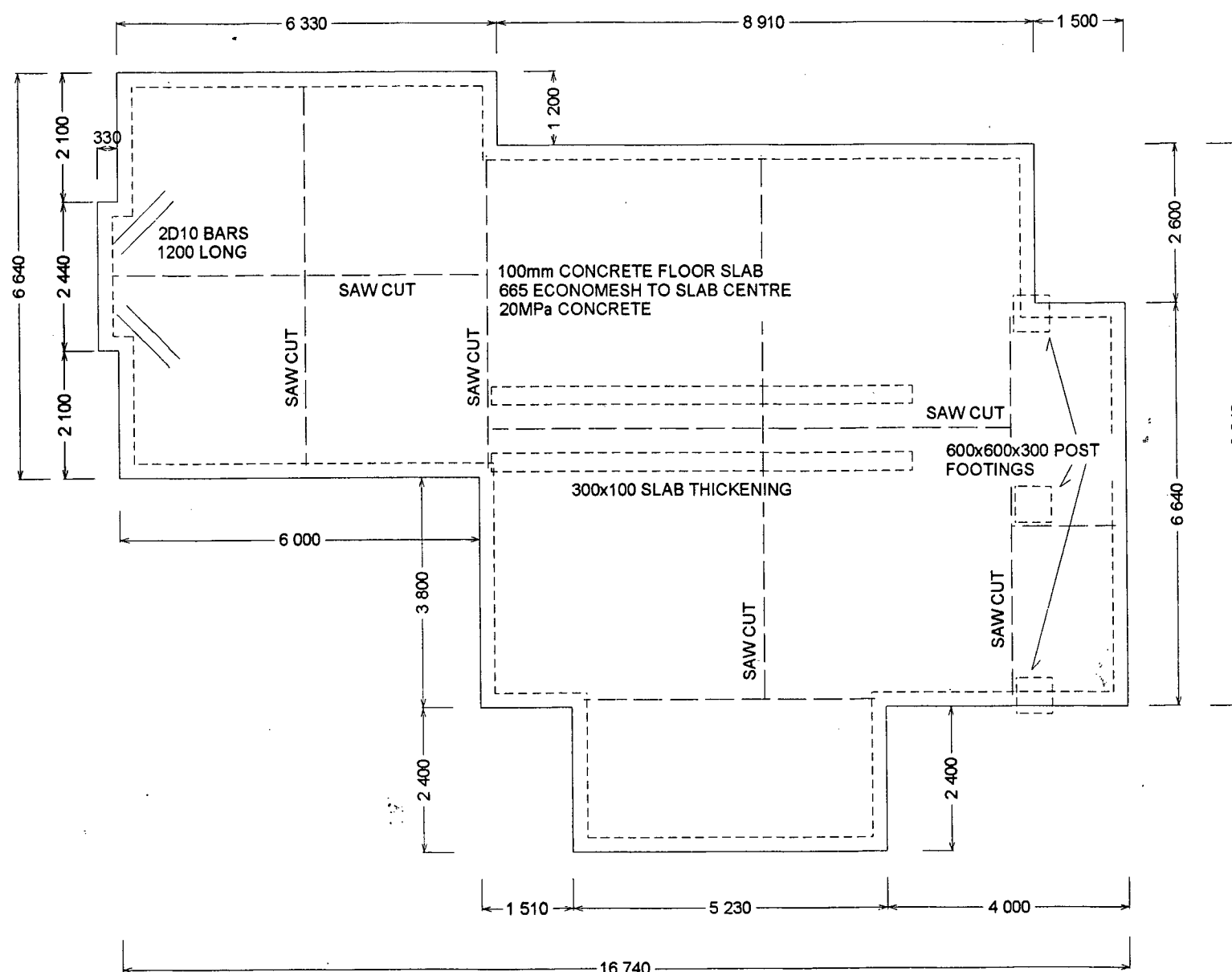
FOUNDATION PLAN
