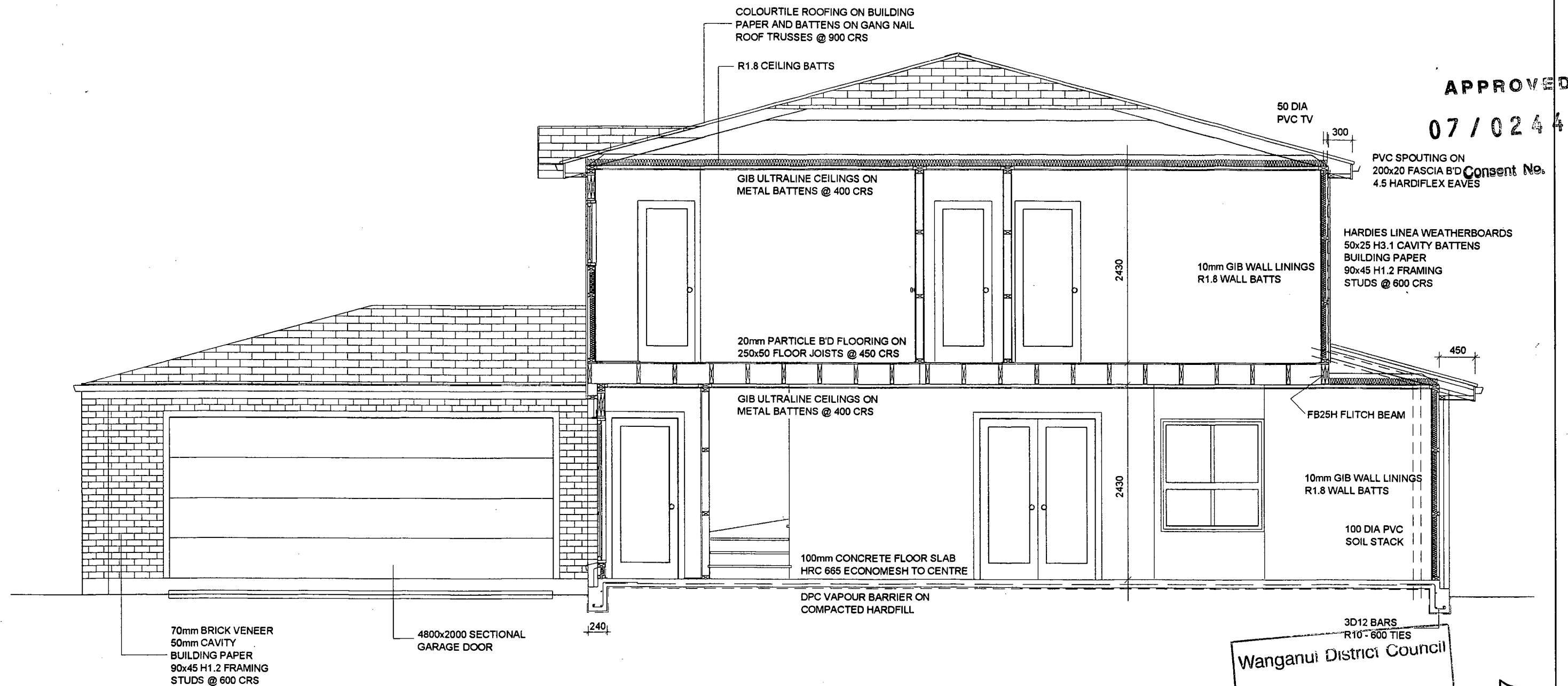
CROSS SECTION HOUSE A HOUSE B SIMILAR
